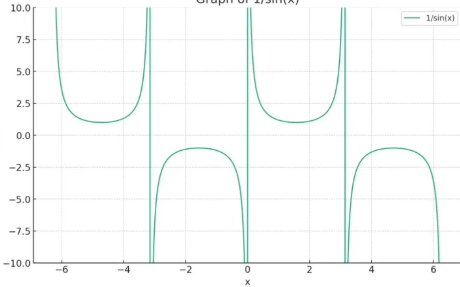
Graph of 1/\sin(x)
